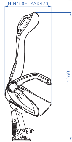
TECHNICAL DRAWING (SIDE VIEW)
