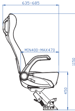
TECHNICAL DRAWING (SIDE VIEW)
